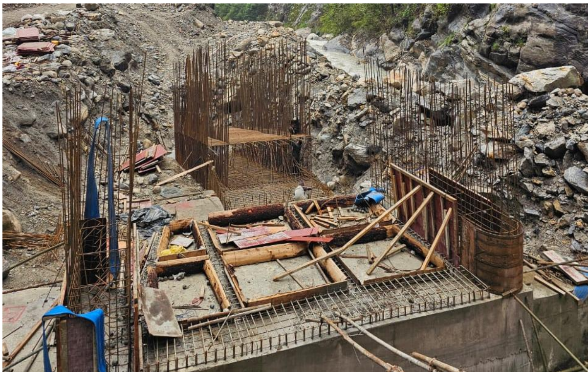
Figure 1: Rebar work in Undersluice gated panel in Headworks
